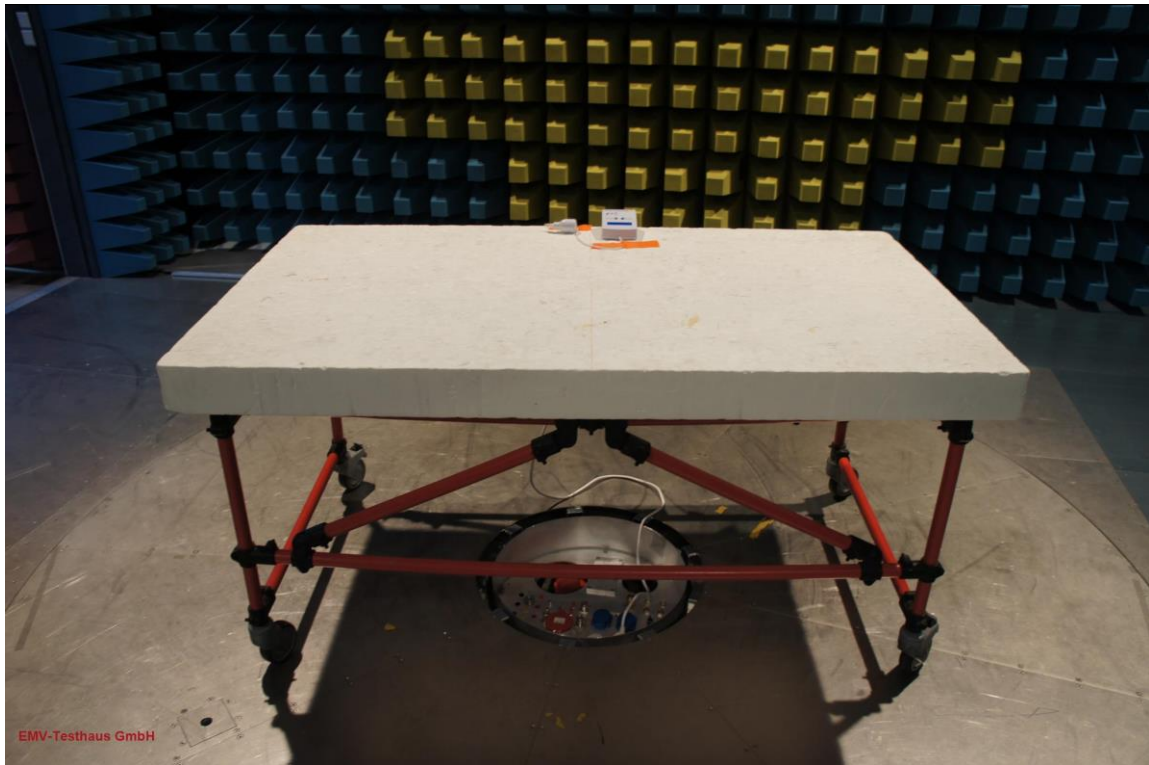
Picture 1: EUT test setup radiated emission test (front view)
