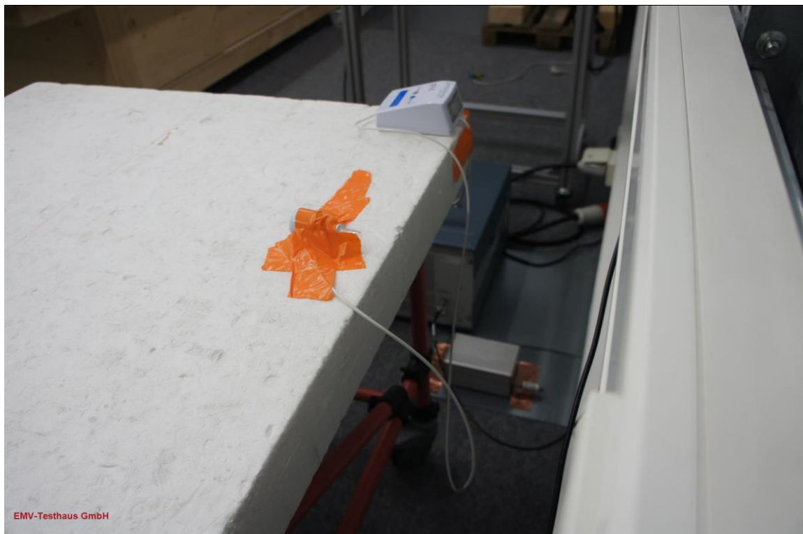
Picture 4: EUT test setup conducted emission test (rear view)
